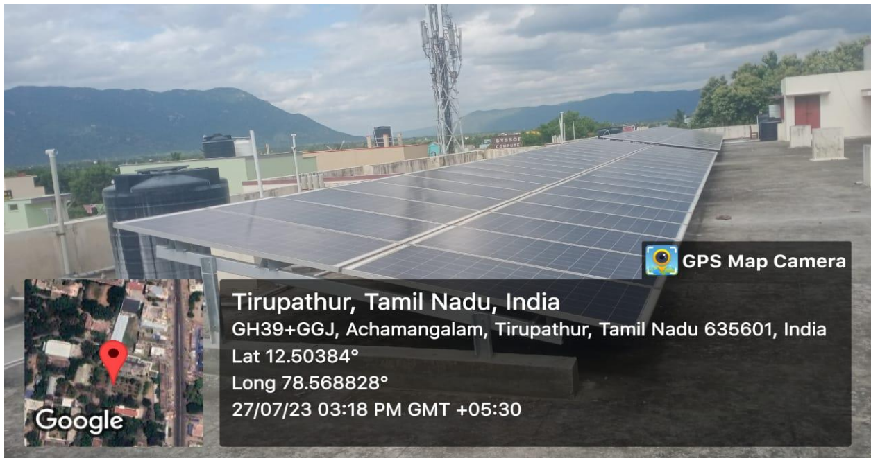
Solar Panels installed in John Med Block
